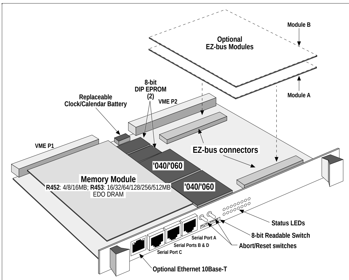
V452 configuration
