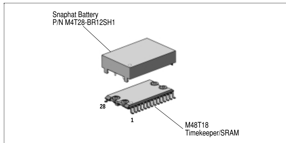
Timekeeper battery removal/installation
