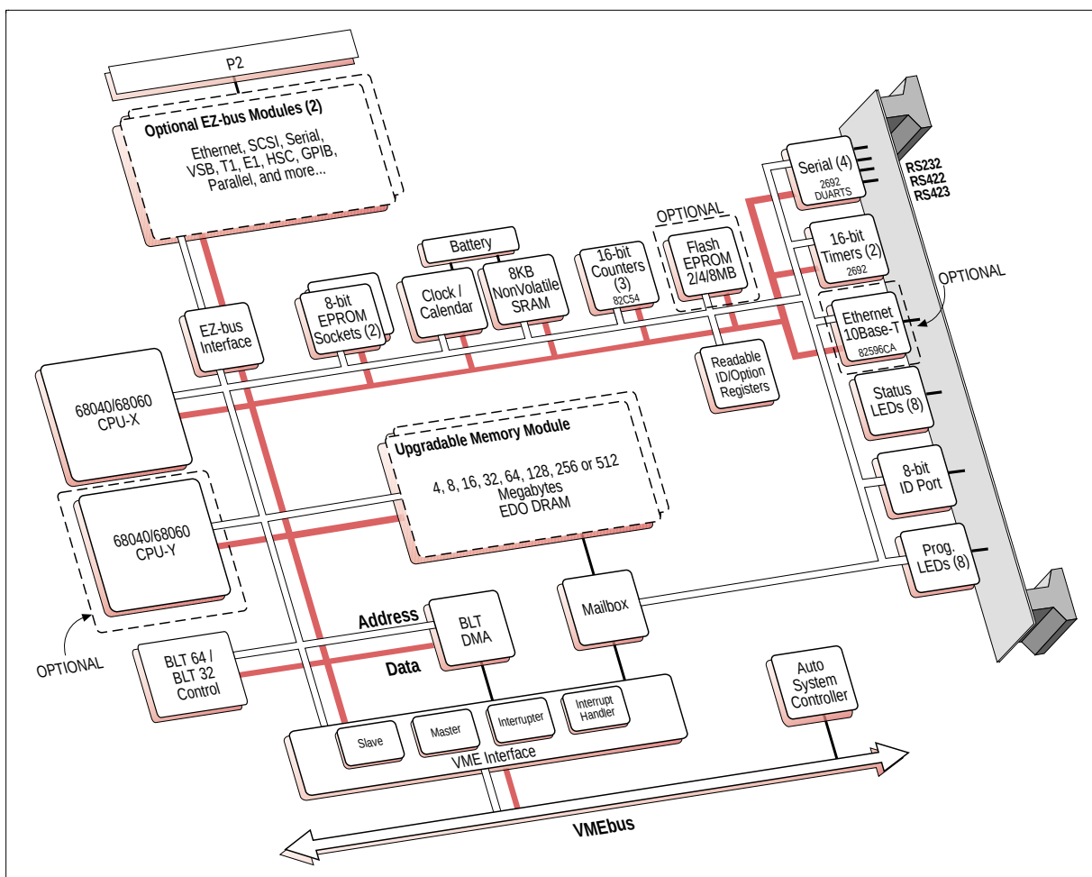
V452 functional block diagram
