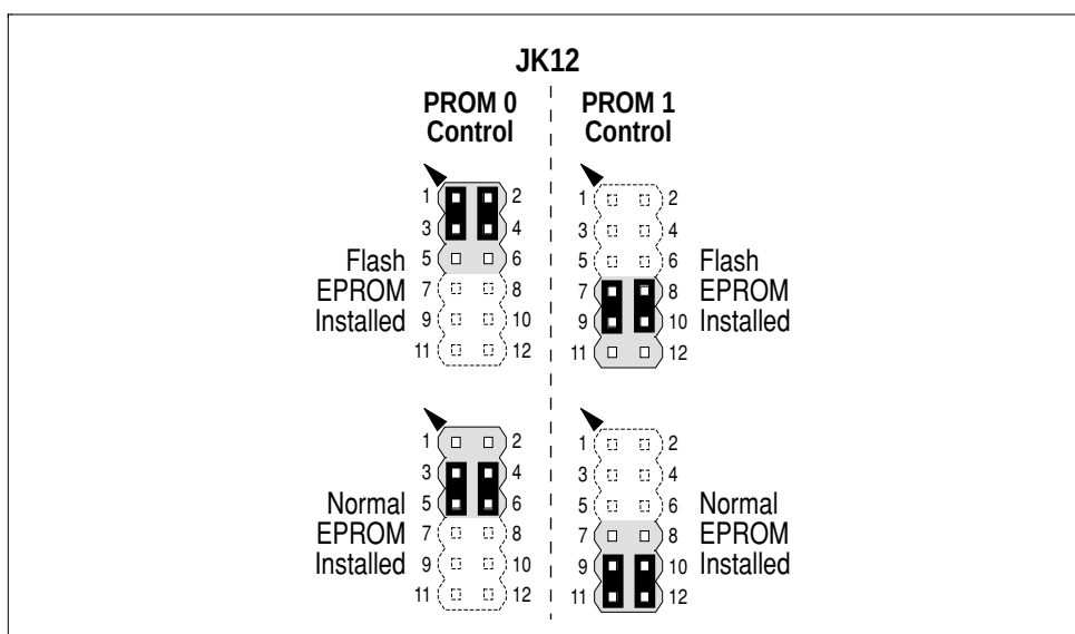
JK12 – EPROM type selection
