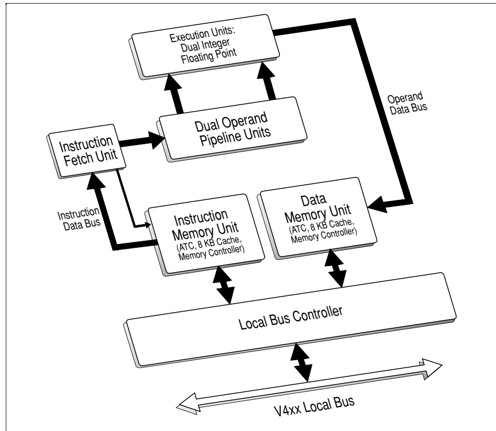
Simplified 68060 block diagram
