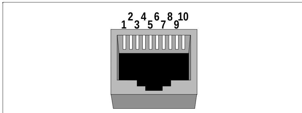
Asynchronous serial connector pin numbering
