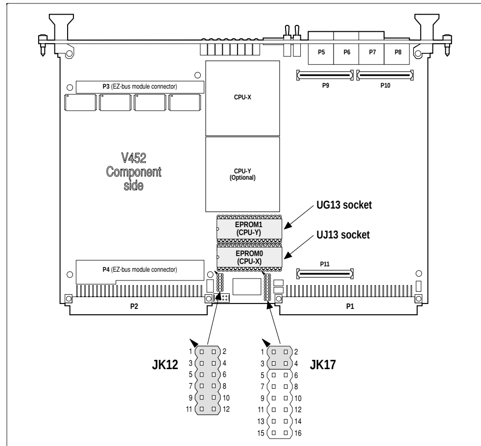
V452 Series jumper and socket locations for EPROM configuration
