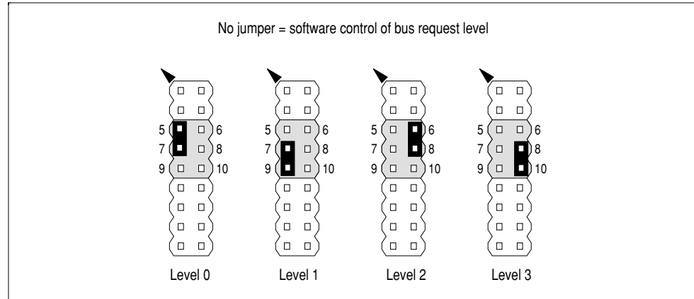
Bus request level jumper settings (JK17)
